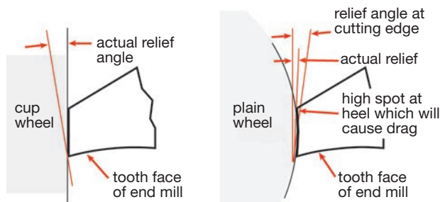
Effect of Wheel Shape on End Mill Relief Angle Cup Wheel versus Plain Wheel
